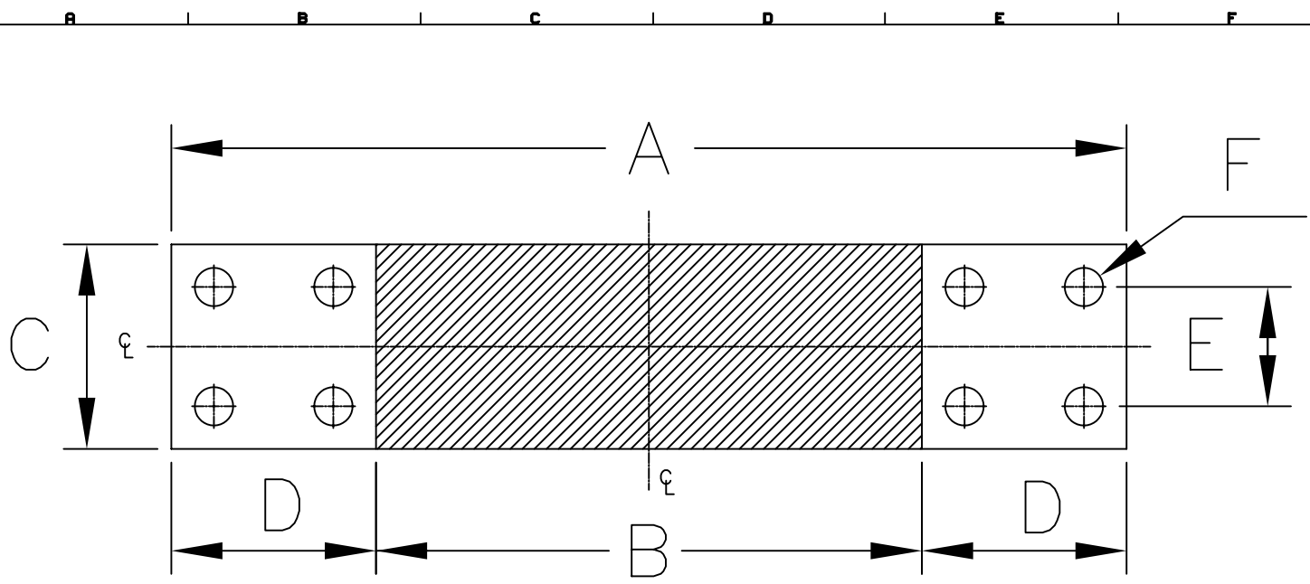
PLAN VIEW
